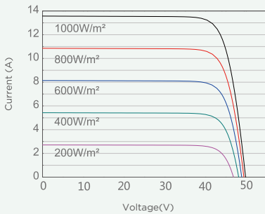
Current-Voltage Curve(SP540M-72H)
