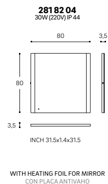
◆ DOUBLE LATERAL LED LIGHT MIRROR W/LOWER LED LIGHT ESPEJO CON DOBLE ILUMINACIÓN LED LATERAL Y LED INFERIOR
