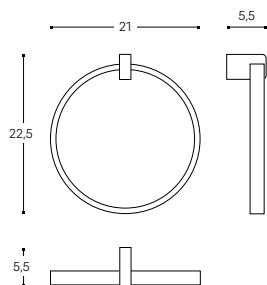
TOWEL RING TOALLERO ARO
