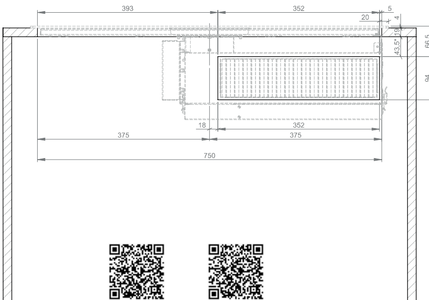
Vista Trasera / Rear view
