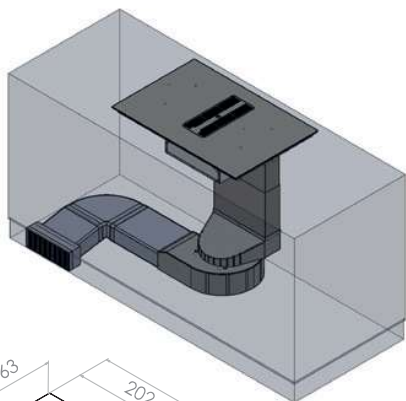
SALIDA FRONTAL FRONT EXIT
