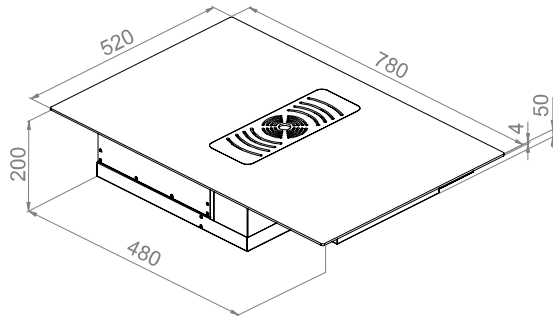
Vista frontal / Front view
