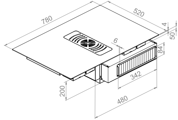
Vista Trasera / Rear view
