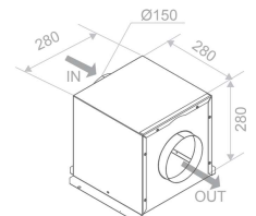
Caja motor remota Box remote engine
